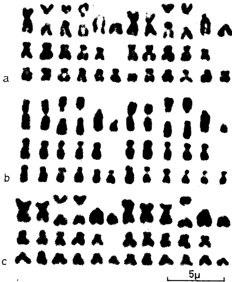
Fig. 9a-c. The diploid karyotypes of Pheidole nodus . a The karyotype having three metacentrics, 2n=39 . b The karyotype having four metacentrics, 2n=38 . c The karyotype having five metacentrics, 2n=37 .
