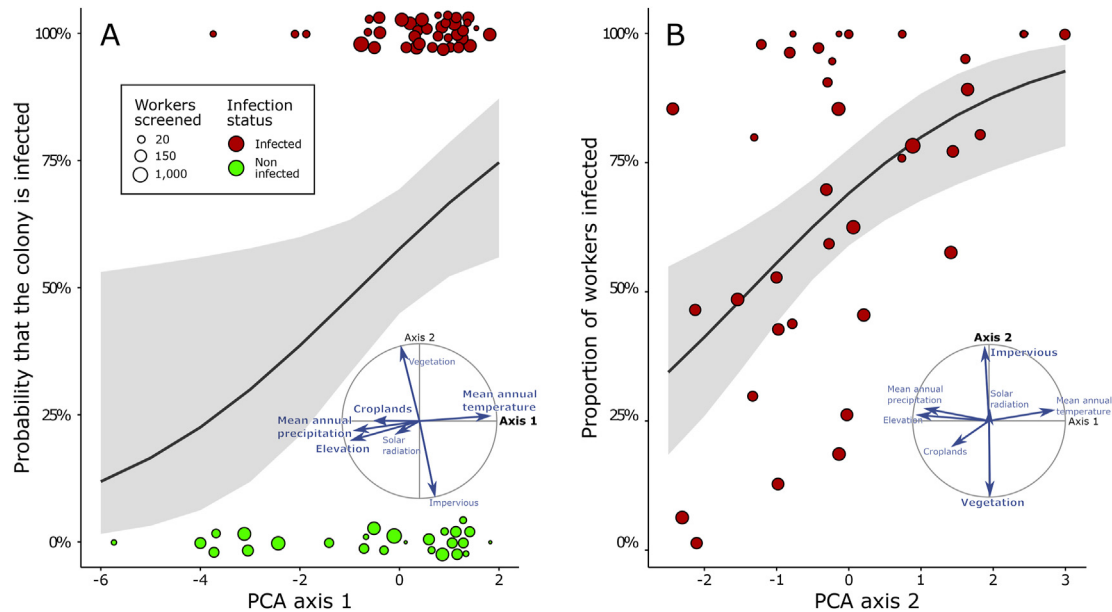
Fig. 4. (A) Relationship (mean \pm 95% CI) between environmental conditions (PCA axis 1) and the probability of Las. neglectus colonies to be infected by Lab. formicarum ( N = 66 colonies, observed values are 0 or 100% but slightly shifted for visual purpose). As illustrated by the bottom-right circle of correlations, the first PCA axis represents a gradient of temperature and precipitation. (B) Relationship (mean \pm 95% CI) between environmental conditions (PCA axis 2) and Lab. formicarum prevalence in infected Las. neglectus colonies ( N = 38 colonies). As illustrated by the bottom-right circle of correlations, the second PCA axis represents a gradient of urbanization as it is negatively correlated with the proportion of vegetated areas and positively correlated to the proportion of impervious surfaces (e.g., buildings, roads).
