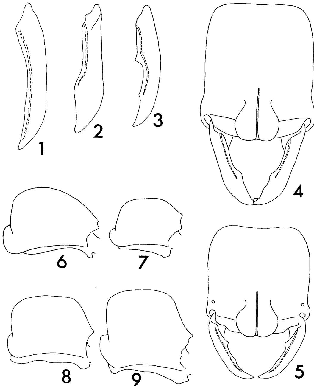
FIGS 1-3. Dorsal view of left mandibular blade in workers, hairs omitted. 1. macgeei , 2. hastifer , 3. minor , showing characteristic shape of mandible in the genus. FIG. 4. Dorsal view of head of anops , pubescence and antennae omitted. FIG. 5. Dorsal view of head of cryptica , pubescence and antennae omitted. FIGS 6-9. Lateral view of petiole in workers. Anterior face to the right; pilosity omitted. 6. hastifer , 7. anops , 8. macgeei , 9. minor .
